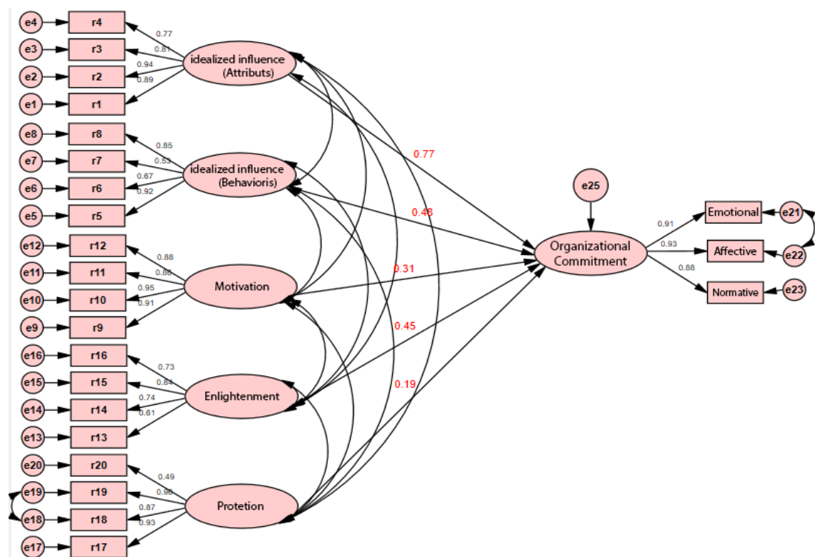
Figure 2. Structural equation model explaining the effect of transformational leadership on organizational commitment
